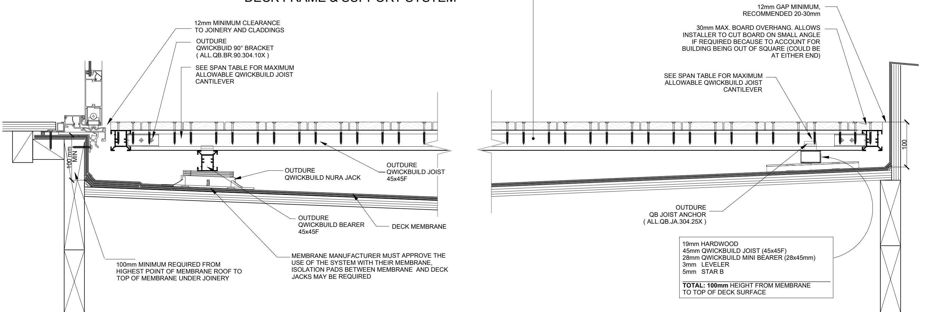
1 QB -H2 100mm LOW HEIGHT HARDWOOD ELEVATION SCALE 1:5
