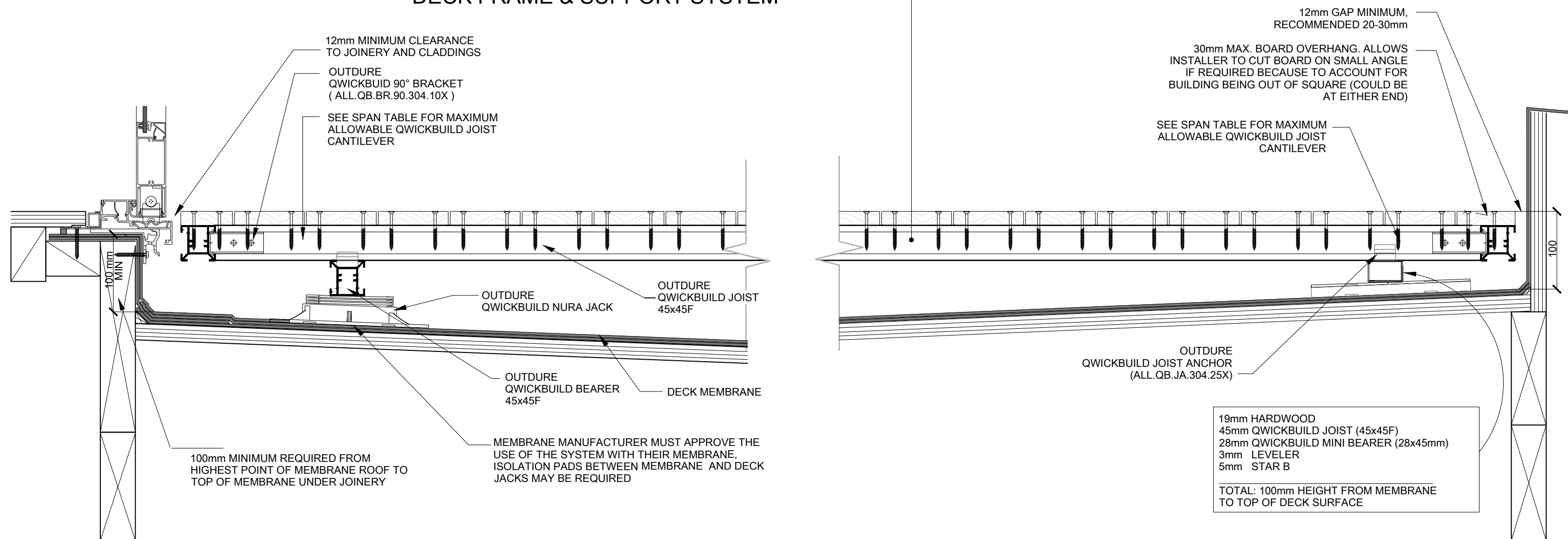
1 QB -H4. HARDWOOD ON MEMBRANE SCALE 1:5
