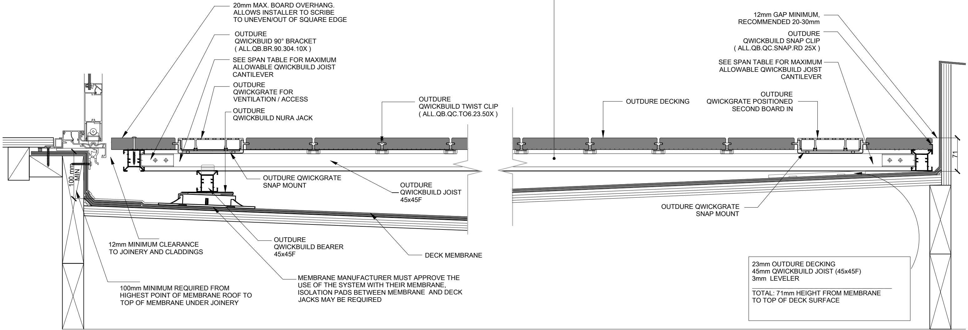
1 QB -OD1. 71mm LOW HEIGHT ELEVATION SCALE 1:5
