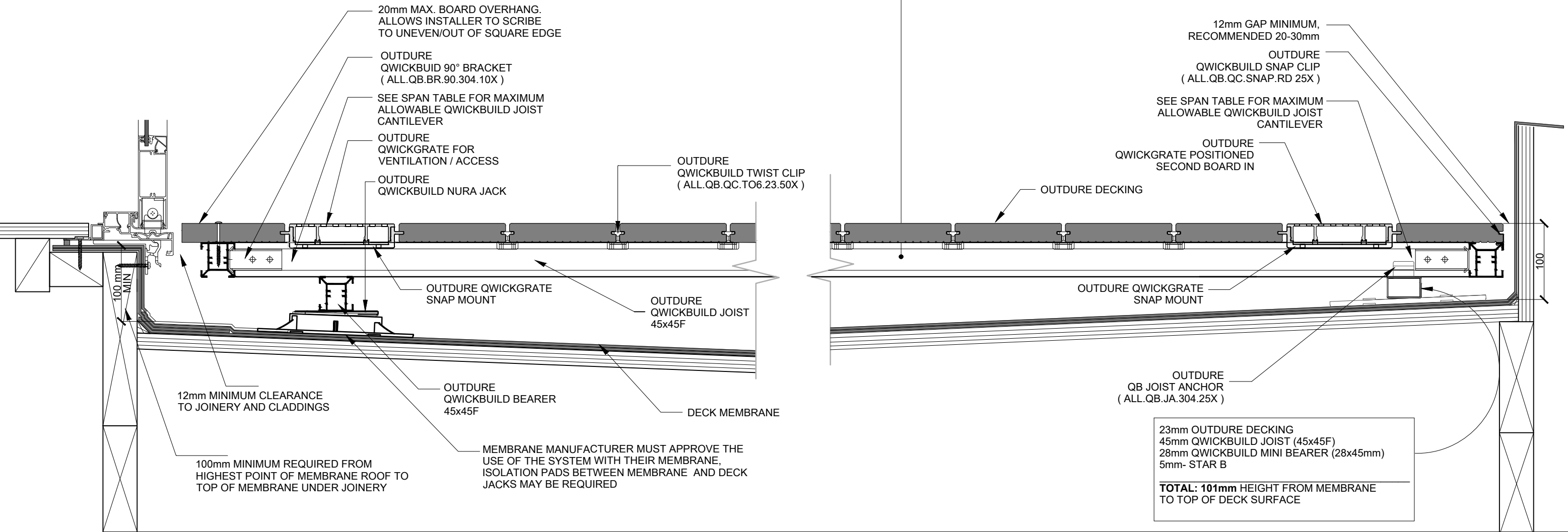
1 QB -OD2. 100mm LOW HEIGHT ELEVATION SCALE 1:5
